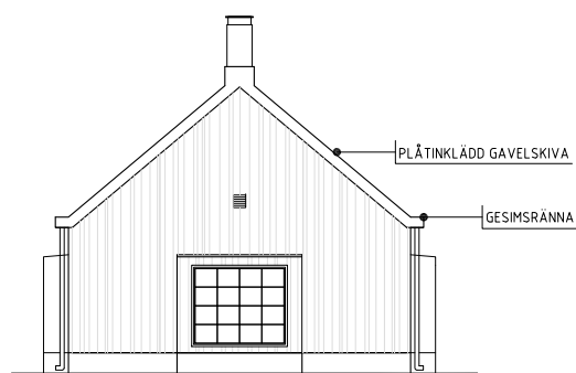
GAVELFASAD
